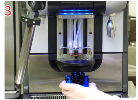
3 Remove the brewing head from the machine.
